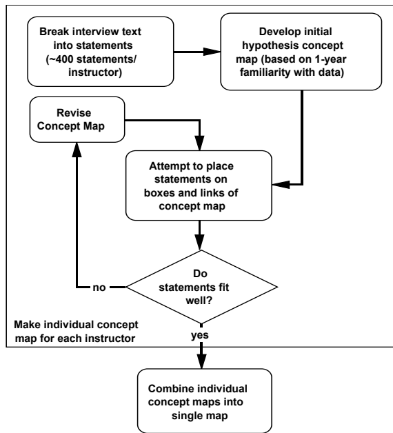
Figure 1: Analysis Procedure
