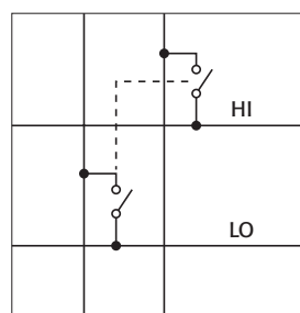
Matrix Crosspoint
